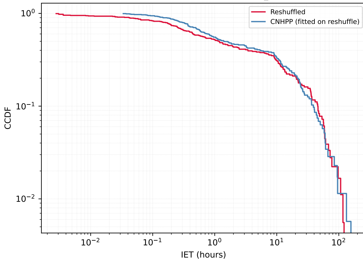
User 53034376 - Reshuffled vs CNHPP A_{\text{fit}}=0.5372
